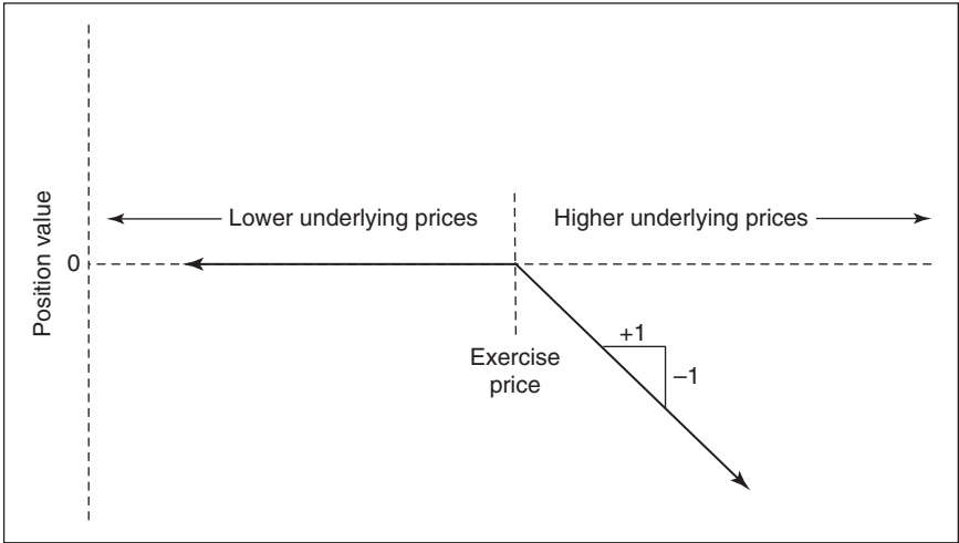
Figure 4-2 Short call.
