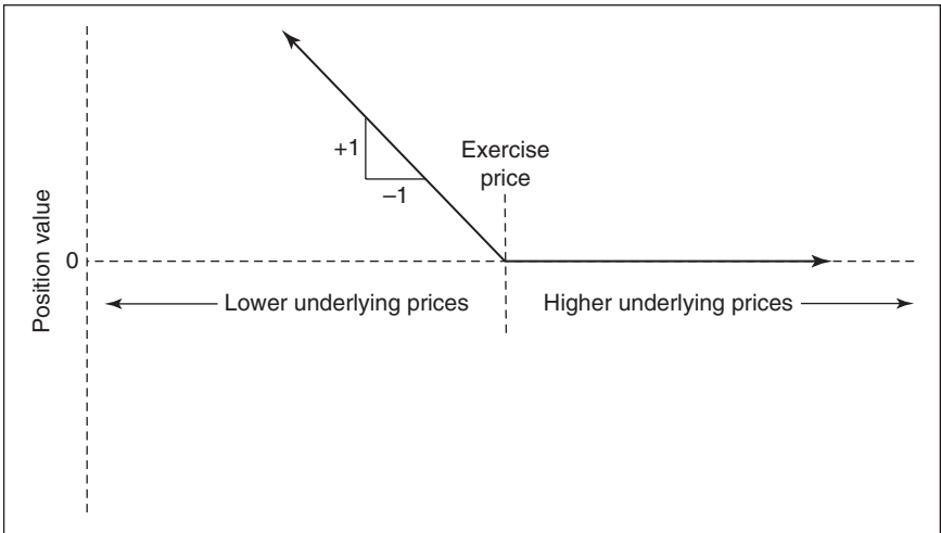
Figure 4-3 Long put.
